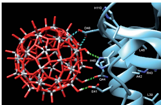
Fig. 3 Model showing the docking of the metal-oxygen core of \text{H}_6[\text{Ti}_{42}(\mu_3\text{-O})_{60}(\text{O}^i\text{Pr})_{42}(\text{OH})_{12}] with the structure of nsp1 taken from 7K7P. 22,39 The possible interactions are shown in cyan: carboxylate of D48 with titanium, forming an inner sphere complex, and green: hydrogen bonding of OH-groups from the nanoparticle to E41, Q44 and H45. The amino acids of the other amides showing chemical shift perturbation are marked.
