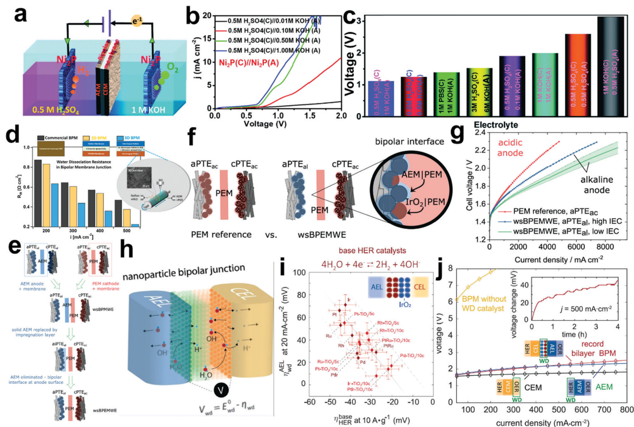
Fig. 19 (a) Schematic illustration of an acid/alkaline asymmetric electrolyte water electrolyzer with \text{Ni}_2\text{P} as the HER and OER electrodes and BPM under a forward bias. (b) The effect of anodic KOH concentration on the polarization curves in the presence of 0.5 \text{ M H}_2\text{SO}_4 . (c) The voltage at 10 \text{ mA cm}^{-2} under different combinations of electrolytes in the cathodic (C) and anodic (A) compartments. (a–c) Reproduced from ref. 319 with permission from the Royal Society of Chemistry. (d) The comparison of resistance ( R_w ) of water dissociation in the interfacial junction for different BPMs at different current densities. Reprinted with permission from ref. 320. Copyright 2020 American Chemical Society. (e) The evolution from BPM water electrolysis MEA configuration (wsBPMWE) with a solid AEM to a new MEA configuration with an AEM impregnation layer in direct contact with the PEM indicating the decrease of AEM thickness. (f) The structure of wsBPEMWE MEAs comprising an anodic porous transport electrode with an alkaline ionomer (aPTE al ), a PEM, and a cathodic porous transport electrode with an alkaline ionomer (cPTE al ) with a variation of the ion-exchange capacity (IEC) of the Aemion binder in the aPTE al compared to a PEM reference consisting of aPTE ac , PEM and cPTE ac with an acidic ionomer binder of Nafion 212. (g) The polarization curves of different MEA configurations. The green area represents the confidence interval obtained from the standard deviation of three individual MEAs of the low IEC system. (e–g) Reprinted with permission from ref. 321. Copyright 2020 American Chemical Society under a license of CC-BY-NC-ND. (h) Different nanoparticles as water dissociation (WD) catalysts loaded on both the acidic CEL and basic AEL surfaces in the BPM interfaces. (i) The overpotentials for WD in a locally basic environment with \text{IrO}_2 used as the stable WD catalyst on the acidic CEL surface correlate with the overpotentials measured for HER in 1 \text{ M KOH} for selected nanoparticles coated on the basic AEL surfaces, consistent with the WD rate limiting the alkaline HER. (j) The polarization curves of PEM, AEM and BPM water electrolyzers. The BPM interface contains either no WD catalysts or \text{NiO} encapsulated by 10 layers of \text{TiO}_2 at the AEL surface and \text{IrO}_2 at the CEL interface. (h–j) Reprinted with permission from ref. 322. Copyright 2020, AAAS.
