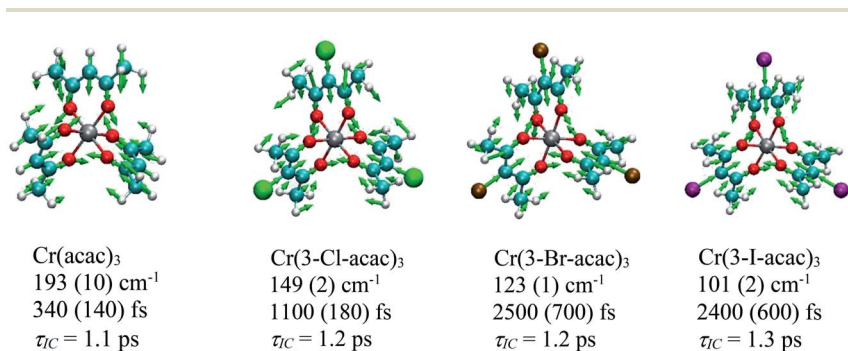
Fig. 13 Nuclear displacements associated with the coherent oscillations identified for the \text{Cr}(3\text{-R-acac})_3 derivatives. Below each compound's name is listed the DFT calculated frequency associated with the coherence feature, the measured dephasing time, and the time constant corresponding to the observed kinetics for excited-state evolution based on the model shown in Fig. 9.
