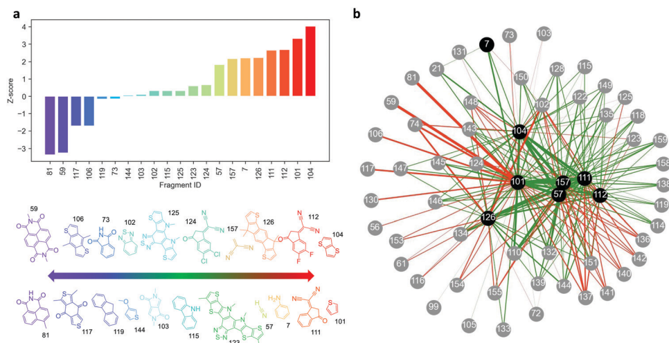
Fig. 3 (a) Z-scores obtained from the discrete hypergeometric distribution of moieties in the highly-absorbing molecules ( f_{osc,max} > 2.5 ) with respect to the entire molecular dataset, for moieties activated at least 10 times. The corresponding structures of identified moieties are shown. (b) Network graph of Z-scores relating pairs of moieties. Source nodes are coloured in black whereas child nodes are coloured in grey. The colour of the edges corresponds to the sign of the Z-score (green for positive, red for negative). The width of the edges scales with the absolute value of the Z-score.
