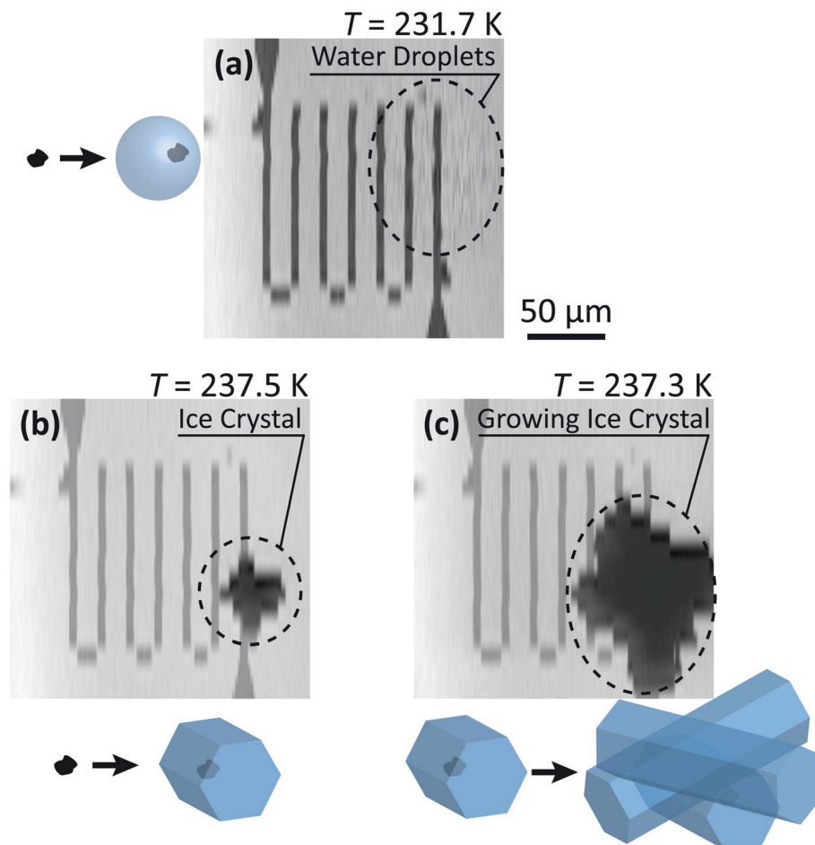
Fig. 4 Example of an INXCell experiment in which (a) water droplets formed, following by (b) ice formation (c) and crystal growth on dry deposited ferrihydrate particles. The temperature, T , of the sample is indicated above the STXM images. The coarse spatial resolution was necessary to quickly image the nucleated and growing ice crystal.
