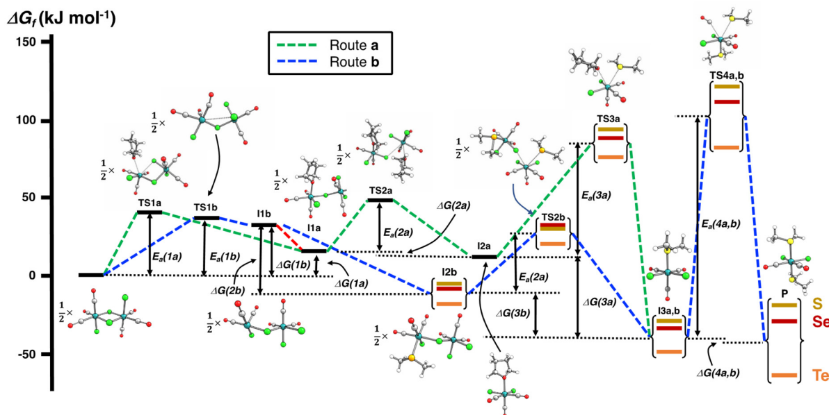
Fig. 4 PBE0-D3/def2-TZVP energy profiles of two alternative routes of the reaction of [\text{RuCl}_2(\text{CO})_3]_2 and \text{EMe}_2 ( \text{E} = \text{S}, \text{Se}, \text{Te} ) in THF. The numerical values of the energetics are shown in Table 2.
