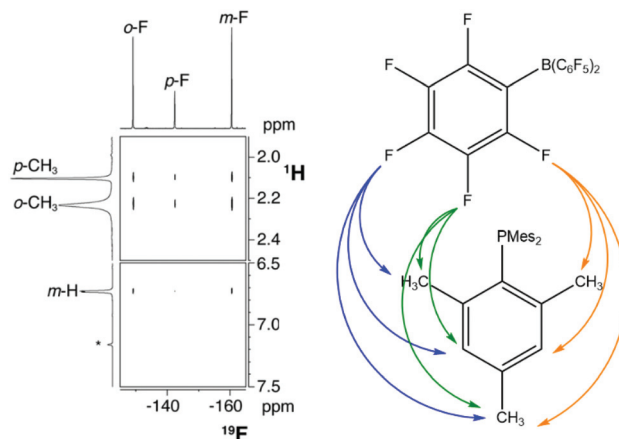
Fig. 3 ^{19}\text{F} , ^1\text{H} HOESY NMR spectrum of \text{PMes}_3/B(\text{C}_6\text{F}_5)_3 in \text{benzene-}d_6 , showing cross-peaks arising from all fluorine and proton environments. Adapted with permission from ref. 68. Copyright 2014 American Chemical Society.
