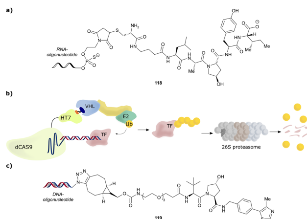
Fig. 50 Oligonucleotide-containing PROTACs. Schematic peptide-based RNA-PROTAC 118 (a), 209 mode of action of TRAFTACs as TF degradation technology (b) 210 and schematic DNA-nucleotide containing TF degrader 119 (c). 211
