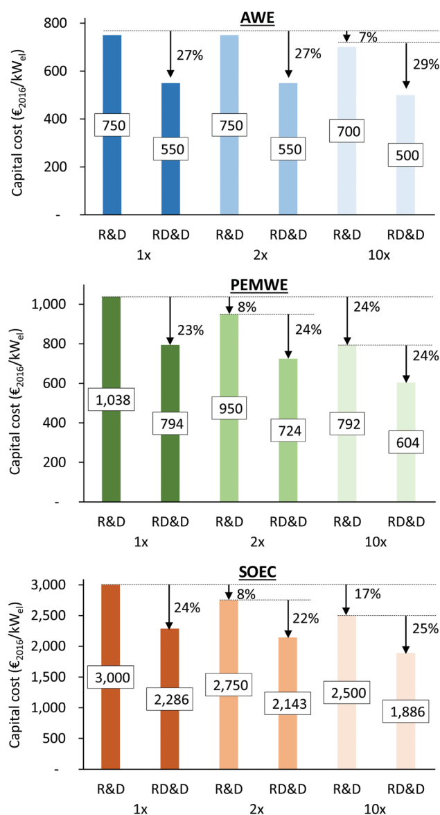
Fig. 166 Estimated capital costs for water electrolysis in 2030 from expert elicitations conducted by Schmidt et al. 1930 . The median cost from all experts is given by technology (top to bottom). Each panel shows the relative impact of increased R&D funding (1x, 2x, 10x) by bars labelled R&D. This impact combined with production scale-up due to increased deployment is shown by bars labelled RD&D. Reproduced from ref. 1930.
