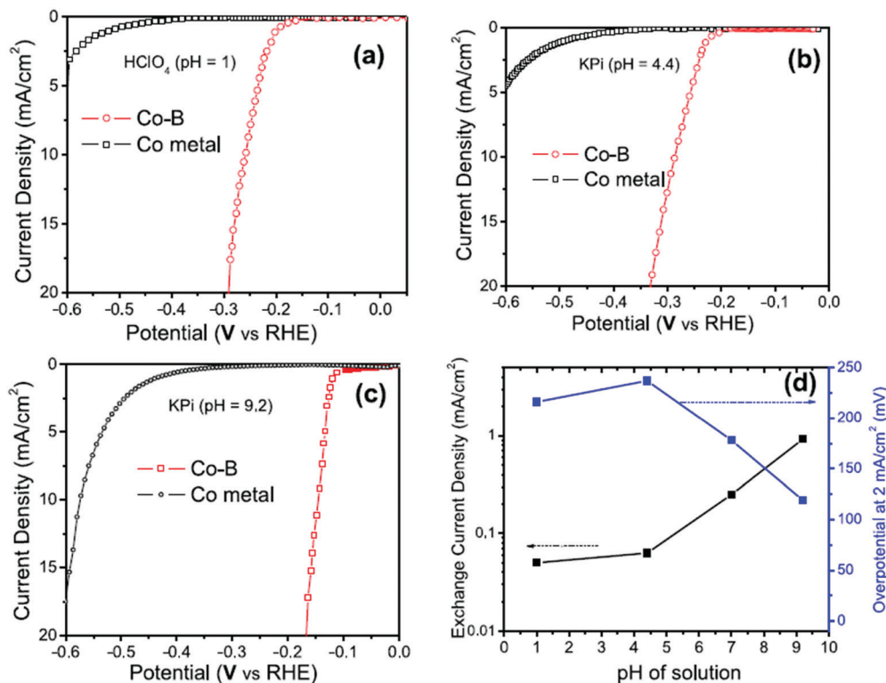
Fig. 55 Linear polarisation curves with iR correction for CoB catalyst compared with Co metal in (a) pH 1 (0.1 M \text{HClO}_4 ), (b) pH 4.4 (0.5 M \text{KH}_2\text{PO}_4 ) and (c) pH 9.2 (0.4 M \text{K}_2\text{HPO}_4 ) obtained with scan rate of 10 \text{ mV s}^{-1} . (d) Plot of overpotential (at 2 \text{ mA cm}^{-2} ) and exchange current density values as a function of pH values of the solution used to test the CoB catalyst. Reproduced with permission from ref. 941. Copyright Wiley 2019.
