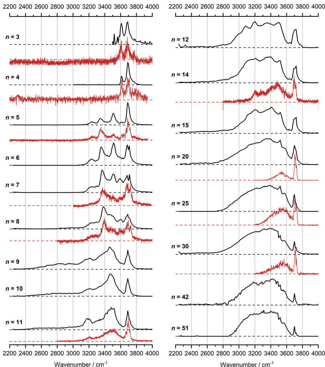
Fig. 1 Infrared multiple photon dissociation spectra of the V^+(\text{H}_2\text{O})_n complexes ( n = 3 – 12 , 14 , 15 , 20 , 25 , 30 , 42 and 51 ) presented in black. For comparison, infrared spectra from Duncan and coworkers are also presented in red for cluster sizes n = 3 – 5 , 7 , 8 , 11 , 14 , 20 , and 30 . 62
