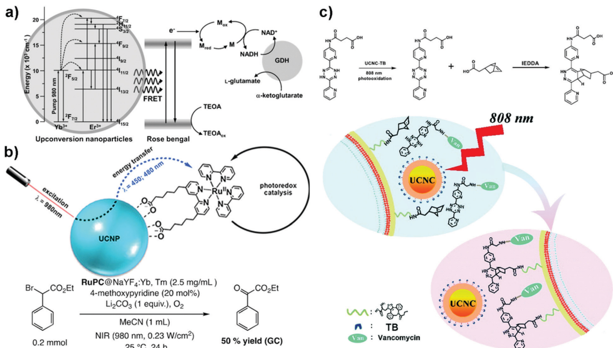
Fig. 3 (a) NIR-driven photoenzymatic catalysts combining \text{NaYF}_4\text{:Yb}^{3+}, \text{Er}^{3+} , Rose Bengal (RB), a rhodium(III)-based mediator (M), nicotinamide adenine dinucleotide ( \text{NAD}^+ ) and L-glutamate dehydrogenase (GDH). 15 Reprinted with permission from ref. 15. Copyright 2014, Wiley-VCH. (b) NIR-driven photocatalyst combining \text{NaYF}_4\text{:Yb}^{3+}, \text{Tm}^{3+} and a heteroleptic derivative of [\text{Ru}(\text{bpy})_3]^{2+} . 16 Reprinted with permission from ref. 16. Copyright 2018, Wiley-VCH. (c) NIR-driven photocatalyst combining \text{NaYF}_4\text{:Nd}^{3+}, \text{Yb}^{3+}, \text{Er}^{3+} and \text{NaYF}_4\text{:Nd}^{3+} and Toluidine Blue O (TB). 17 Reprinted with permission from ref. 17. Copyright 2021, Royal Society of Chemistry.
