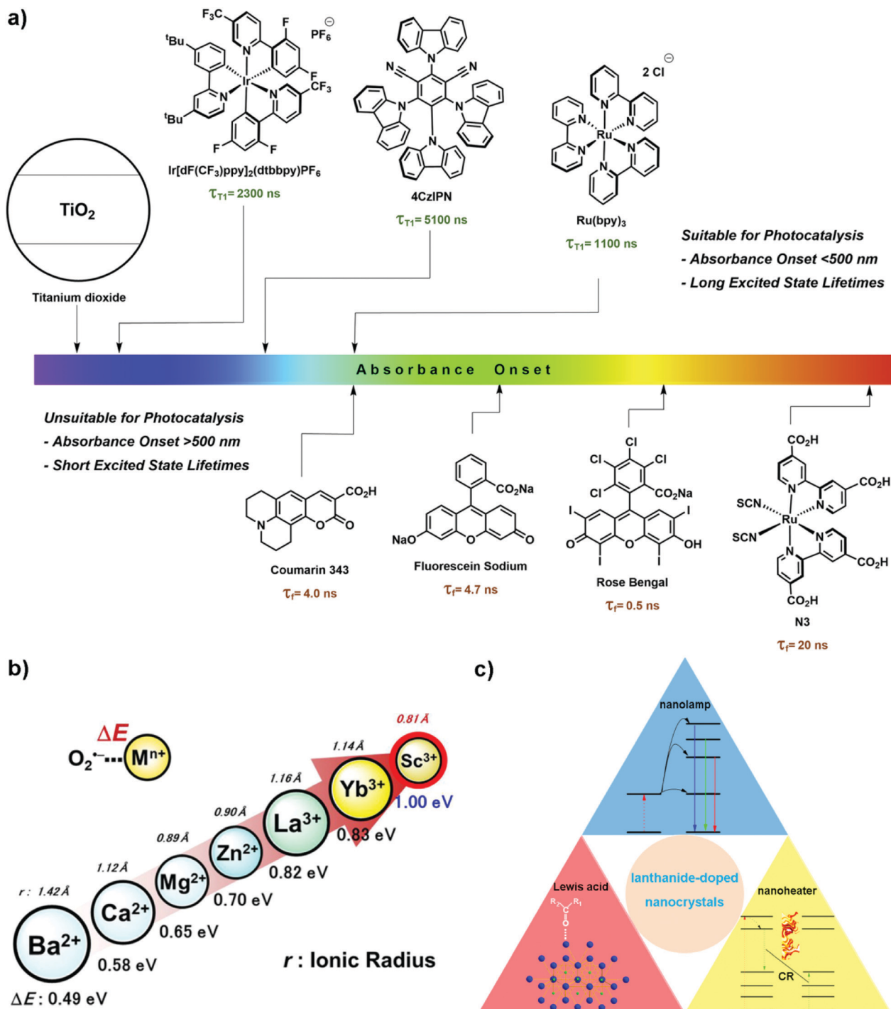
Fig. 1 (a) Absorption window of photosensitizers including dyes and semiconductors. 35 Reprinted with permission from ref. 35. Copyright 2021, Elsevier. (b) The relationship between the Lewis acidity ( \Delta E ) and ionic radius of redox-inactive \text{Re}^{3+} ions. 51 Details of the measurement of \Delta E can be found in ref. 51. Reprinted with permission from ref. 51. Copyright 2017, Wiley-VCH. (c) Scheme of the three functions (i.e., Lewis acid catalyst, upconversion nanolamp, and photothermal nanoheater) of lanthanide-doped nanocrystals.
