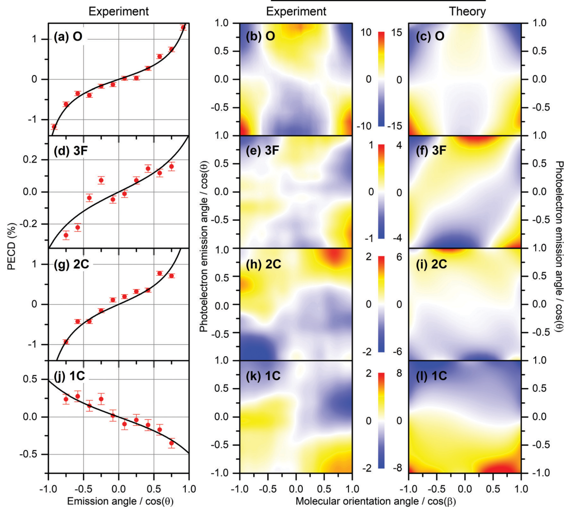
Fig. 2 Experimental and theoretical PECD of R-TFMOx represented as the normalized difference of the electron emission probabilities, obtained for 1s-photoelectrons of the oxygen atom (a–c, O), all three fluorine atoms (d–f, 3F), the two carbon atoms from the oxirane ring (g–i, 2C), and the carbon atom in the trifluoromethyl group (j–l, 1C). Kinetic energy of all photoelectrons is equal to about 11 eV. The left-hand panels (a,d,g,j) illustrate the retrieval of the anisotropy \beta_2 and dichroic \beta_1 parameters by fitting (black curves) the PECD, measured for randomly oriented molecules (red circles), with eqn (2). The middle and the right-hand panels illustrate the experimental (b,e,h,k) and theoretical (c,f,i,l) differential PECD as a function of the photoelectron emission angle \theta and molecular orientation angle \beta between the momentum vector of the \text{CF}_{2,3}^+ fragment and the light propagation direction. The statistical uncertainties, taken at the peak values of the experimental data, are: (b, O) \pm 0.45\% ; (e, 3F) \pm 0.17\% ; (h, 2C) \pm 0.25\% ; and (k, 1C) \pm 0.16\% .
