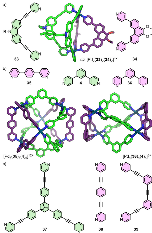
Fig. 8 (a) Geometric complementarity between ditopic ligands 33 and 34 facilitates access to the heteroleptic cage cis\text{-}[\text{Pd}_2(\mathbf{33})_2(\mathbf{34})_2]^{4+} (SCXRD structure). (b) Higher nuclearity heteroleptic structures have also been reported, such as [\text{Pd}_6(\mathbf{35})_6(\mathbf{4})_6]^{12+} and [\text{Pd}_4(\mathbf{36})_4(\mathbf{4})_4]^{8+} (SCXRD structures). (c) Through matching of ligand geometries, in combination with denticity mismatch, trigonal prismatic cages [\text{Pd}_3(\mathbf{37})_2(\mathbf{38}/\mathbf{39})_3]^{6+} have been realised.
