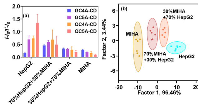
Fig. 4 (a) Changes in fluorescence intensities ( I - I_0/I_0 ) against mixed cells using four CA-CD coassemblies (CA-CD: 4.0/4.0 \mu M, AlPcS 4 : 4.0 \mu M, the number of cells: 1.5 \times 10^4 ). (b) Canonical scores plot for the two factors of simplified fluorescence response patterns obtained with CA-CD/AlPcS 4 array against mixed cell lines (calculated by LDA, 90% confidence). All experiments were in HEPES buffer (10 mM, pH = 7.4) at 25 ^{\circ} C.
