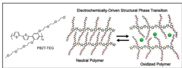
Fig. 8 Chemical structure of PB2T-TEG along with the uncovered unzipping/zippering mechanism for ion insertion. Reproduced with permission from American Chemical Society. 83
