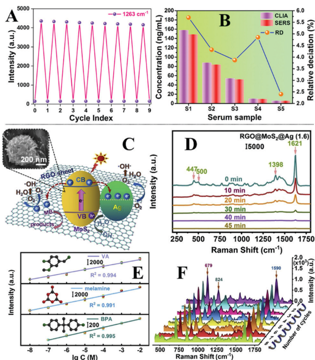
Fig. 16 (A) Plot showing the SERS activity of the \text{Fe}_3\text{O}_4@ \text{TiO}_2@ \text{Ag} micro-particles after 9 cycles of photo-regeneration; (B) plot comparing SERS results obtained from \text{Fe}_3\text{O}_4@ \text{TiO}_2@ \text{Ag} microparticles and chemiluminescent results obtained from commercial immunoassay kits; (C) schematic illustrations of the photodegradation process on \text{RGO}@ \text{MoS}_2@ \text{Ag} nanocomposites. Inset shows the SEM image of a typical \text{RGO}@ \text{MoS}_2@ \text{Ag} particle; (D) SERS spectra showing the photodegradation of methylene blue catalysed by \text{RGO}@ \text{MoS}_2@ \text{Ag} nanocomposites; (E) plots showing the change in SERS signal intensity of melamine, vanillin and bisphenol A in milk as a function of analyte concentration; (F) SERS spectra of a milk sample spiked with a mixture of melamine, vanillin and bisphenol A obtained using the same batch of \text{RGO}@ \text{MoS}_2@ \text{Ag} nanocomposites after 8 cycles of photo-regeneration. Panel (A and B) reproduced with permission from ref. 235, copyright 2020 Elsevier Ltd. Panel (C–F) adapted with permission from ref. 243, copyright 2021 Elsevier Ltd.
