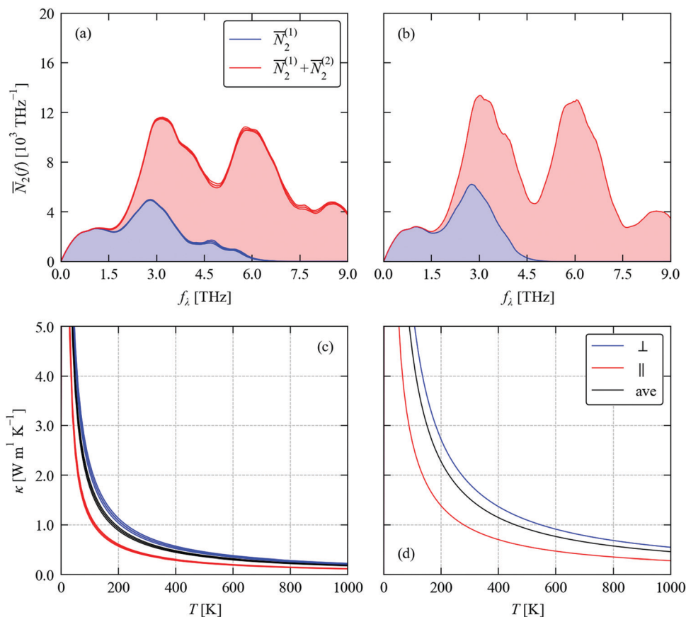
Fig. 9 Thermal conductivity of \text{Sn}(\text{Sn}_{0.1875}\text{Se}_{0.8125}) predicted using the model defined in eqn (8) with the phonon–phonon interaction strengths replaced by a constant value \tilde{P} = 1.469 \times 10^{-12} \text{ eV}^2 . (a) and (b) Two-phonon weighted joint density-of-states functions \tilde{N}_2(\omega) defined in eqn (13). (c) and (d) Predicted in-plane ( \kappa_{\perp} , blue), out-of-plane ( \kappa_{\parallel} , red) and average thermal conductivity ( \kappa_{\text{ave}} , black). Plots (a) and (c) show calculations on the \text{Sn}(\text{Sn}_{0.1875}\text{Se}_{0.8125}) alloy model, and the shaded areas indicate \pm one standard deviation. Plots (b) and (d) show calculations on SnSe for comparison.
