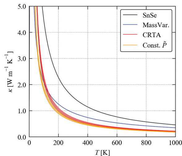
Fig. 10 Predicted averaged thermal conductivity \kappa_{\text{ave}} of SnSe (black) and the \kappa_{\text{ave}} of \text{Sn}(\text{Sn}_{0.1875}\text{Se}_{0.8125}) obtained using the three models considered in this section: the mass-variance model (blue), the CRTA model defined in eqn (3) and (4) with an interpolated lifetime \tau^{\text{CRTA}} (red), and the model defined in eqn (8) with the interaction strengths P_{\lambda} replaced by an interpolated constant \tilde{P} (orange).
