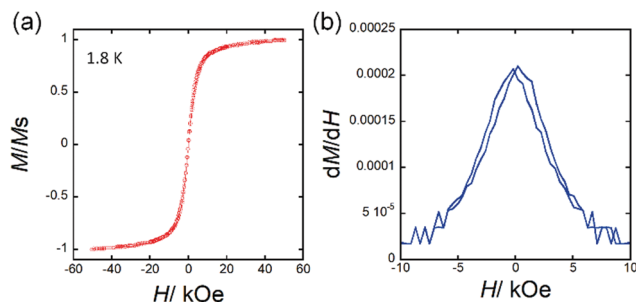
Fig. 4 (a) M - H curve and (b) dM/dH versus H plot for \text{TbPc}_2 @SWCNT at 1.8 K. The vertical axis, M/M_s , shows magnetization values normalized to the saturated magnetization value. The butterfly-type magnetic hysteresis seems to be closed in (a), but it is slightly open which was confirmed by using magnetic field differentiation of M in (b). The lines are guides for eyes.
