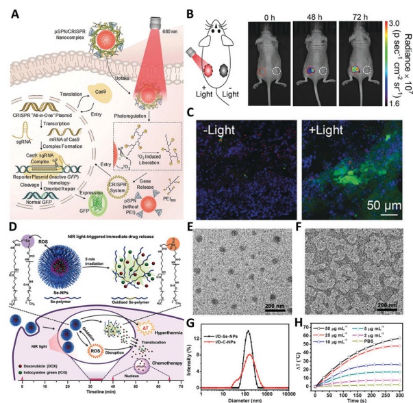
Fig. 4 NIR phototriggered ROS-targeted delivery. (A) NIR phototriggered ROS for on-demand gene editing based on SPN-delivery. (B) Whole-animal fluorescence images at the target location with (left) and without (right) light irradiation (0.3 W cm -2 , 20 min). (C) CLSM images of slices of mice with or without 680 nm irradiation treatment (72 h) (red: pSPN; green: GFP; blue: cell nuclei). Reproduced with permission from ref. 92. Copyright 2019 Wiley-VCH. (D) Selenium-inserted polymeric nanoparticles with tunable hydrophobicity for delivery and synergistic PTT. (E) Representative TEM image of Se-based nanoparticles. (F) The disassembly of Se-based nanoparticles after irradiation (785 nm, 1.0 W cm -2 , 3 min). (G) The size distribution of I/D-Se-NPs and I/D-C-NPs. (H) Temperature elevation of the nanomaterials under irradiation after loading different amounts of ICG. Reproduced with permission from ref. 102. Copyright 2017 American Chemical Society.
