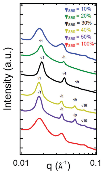
Fig. 4 1D SAXS patterns for the dog bone samples after polymerization and vacuum drying. A transition to LAM is seen with samples \varphi_{\text{SBS}} = 50\% , 40\% , 30\% , and 20\% from the higher-order reflections indexed to the primary scattering peak as indicated on the scattering curves. Scattering plots have been vertically shifted.
