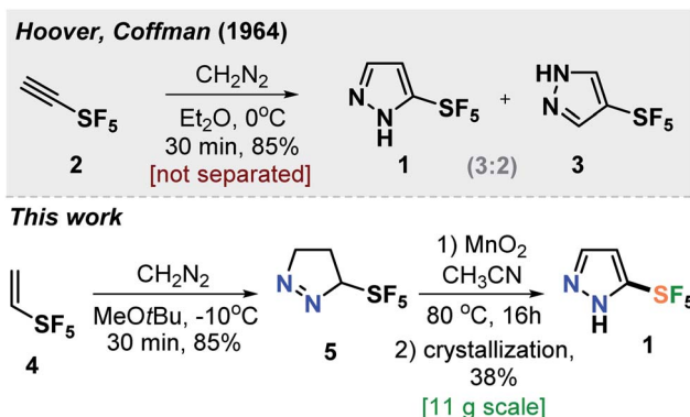
Scheme 1 Synthesis of \text{SF}_5 -pyrazole 1 .
