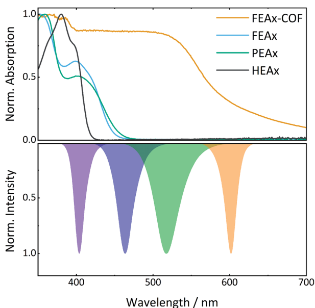
Fig. 3 UV-vis spectra of model compounds and FEAx-COF (top) in comparison to LED emission spectra (bottom).
