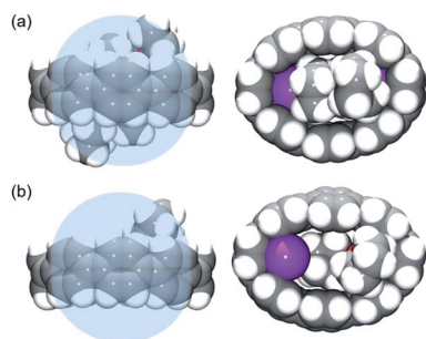
Fig. 4 Comparison of host-guest interactions of 1 4- nanohoop in 2 (a) vs. that in ref. 62 (b), side and face views, space-filling models. The internal space is shown as the blue sphere.
