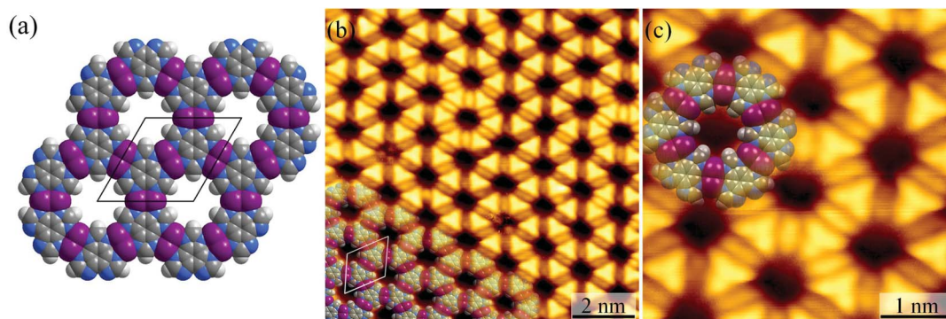
Fig. 3 (a) MM simulated structure of [\text{Ag}_3\text{btim}] . (b) The large-scale ( U = 1.6 \text{ V} , I = 100 \text{ pA} ) and (c) high-resolution ( U = 0.08 \text{ V} , I = 1.54 \text{ nA} ) STM image of [\text{Ag}_3(\text{btim})] on Ag(111) surfaces. The unit cell is indicated in black/white in (a)/(b). Molecular models are superimposed on the respective image.
