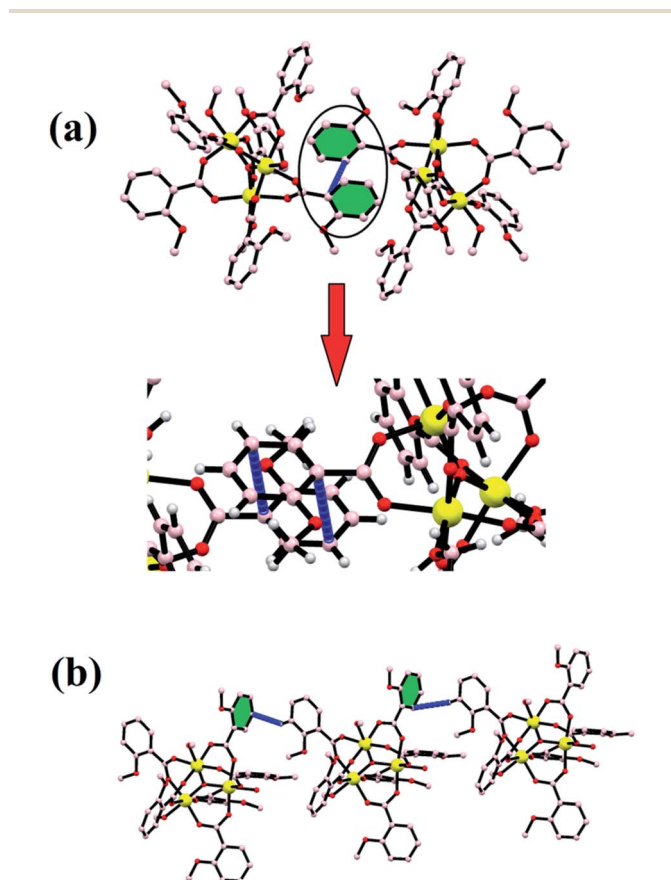
Fig. 3 Stability in the \{\text{Fe}_3\} cluster due to \pi – \pi (a) and C–H \cdots\pi (b) interactions.
