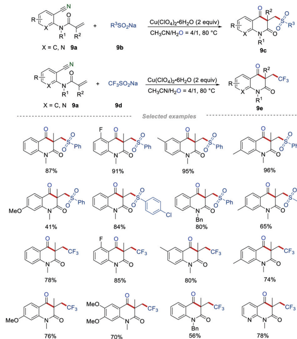
Scheme 9 The construction of sulfonylated and trifluoromethylated quinoline-2,4-diones.
