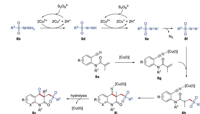
Scheme 8 The construction of sulfonylated quinoline-2,4-diones.
