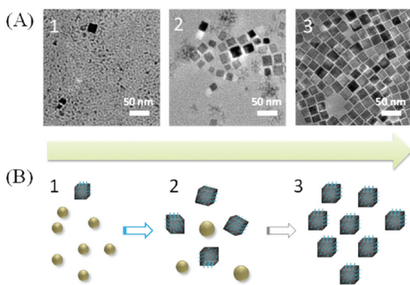
Fig. 14 (A) TEM of the \text{Cu}_3\text{N} NCs synthesized according to ref. 105, after 2, 5 and 10 min. (B) The proposed growth procedure of \text{Cu}_3\text{N} nanocrystals. Reproduced from ref. 105 with permission from the Royal Society of Chemistry.
