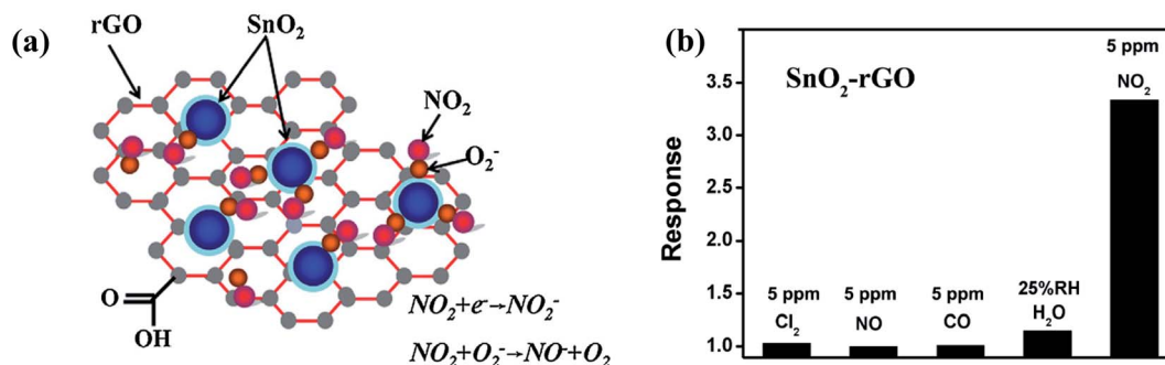
Fig. 7 (a) Illustration of the sensing mechanism for the gas sensor based on SnO 2 /rGO nanostructure. (b) Selectivity (calculated using R_g/R_a ) histogram of SnO 2 /rGO gas sensor to various gases at room temperature. 98 (reprinted from ref. 98, Copyright (2014), with permission from Elsevier).
