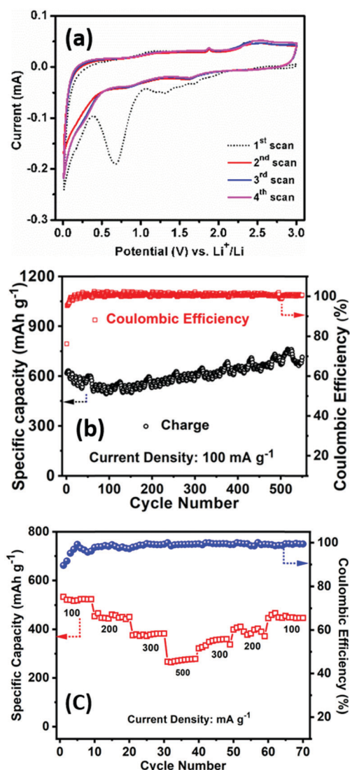
Fig. 5 Electrochemical half-cell LIB anode performance of the PSCNs. (a) Cyclic voltammetry of the PSCN electrode for the first four cycles at 0.1 \text{ mV s}^{-1} at 0.01\text{--}3.0 \text{ V} , (b) cycling performance at 100 \text{ mA g}^{-1} current density, and (c) rate performance at different current densities ( 100\text{--}500 \text{ mA g}^{-1} ).
