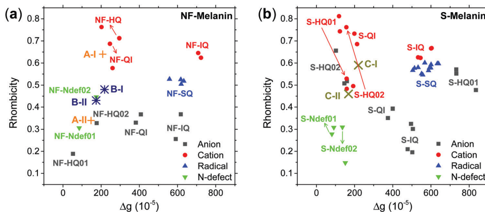
Fig. 5 The plot of the rhombicity as a function of g -anisotropy for the different (a) NF-melanin and (b) S-melanin radical species. The theoretical radicals are represented by the square, circle and triangle symbols; the crosses are each of the experimental radicals. A purely isotropic signal would have \Delta g = 0 and a completely axial symmetry signal would be obtained with rhombicity equal to 1.0 or 0.0.
