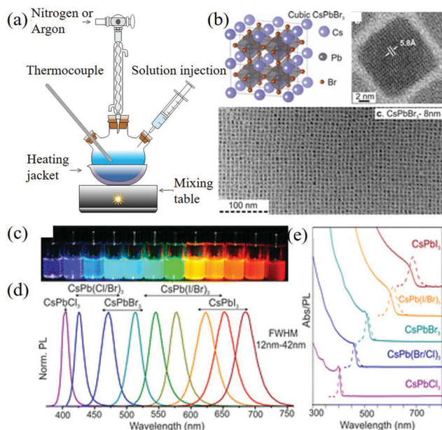
Fig. 3 (a) Colloid quantum dot synthesis device. (b) Schematic of the cubic perovskite lattice and typical transmission electron microscopy (TEM) images of CsPbBr 3 NCs. (c) CsPbX 3 NCs (X = Cl, Br, I) colloidal solutions in toluene under UV lamp ( \lambda = 365 nm). (d) Representative PL spectra ( \lambda_{\text{exc}} = 400 nm for all but 350 nm for the CsPbCl 3 samples). (e) Typical optical absorption and PL spectra (Reproduced from ref. 22 with permission from American Chemical Society).
