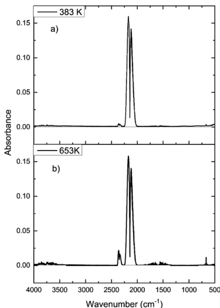
Fig. 11 FTIR spectra for continuous CO dosing over the dried support material (attapulgitite) at (a) 383 and (b) 653 K. Flow conditions: CO 5 \text{ cm}^3 \text{ min}^{-1} , N 2 (carrier gas) 54 \text{ cm}^3 \text{ min}^{-1} , and N 2 (diluent post-reactor) 100 \text{ cm}^3 \text{ min}^{-1} .
