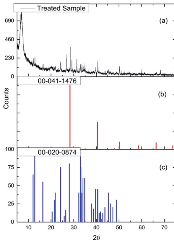
Fig. 15 (a) The X-ray diffraction pattern of the dichlorine pre-treated \text{CuCl}_2/\text{KCl}/\text{attapulgit} catalyst (chlorine exposure = 12.8 mmol \text{Cl}_2 per \text{g}_{(\text{cat})} ). Reference diffraction patterns for (b) KCl (red) and (c) \text{KCuCl}_3 (blue).
