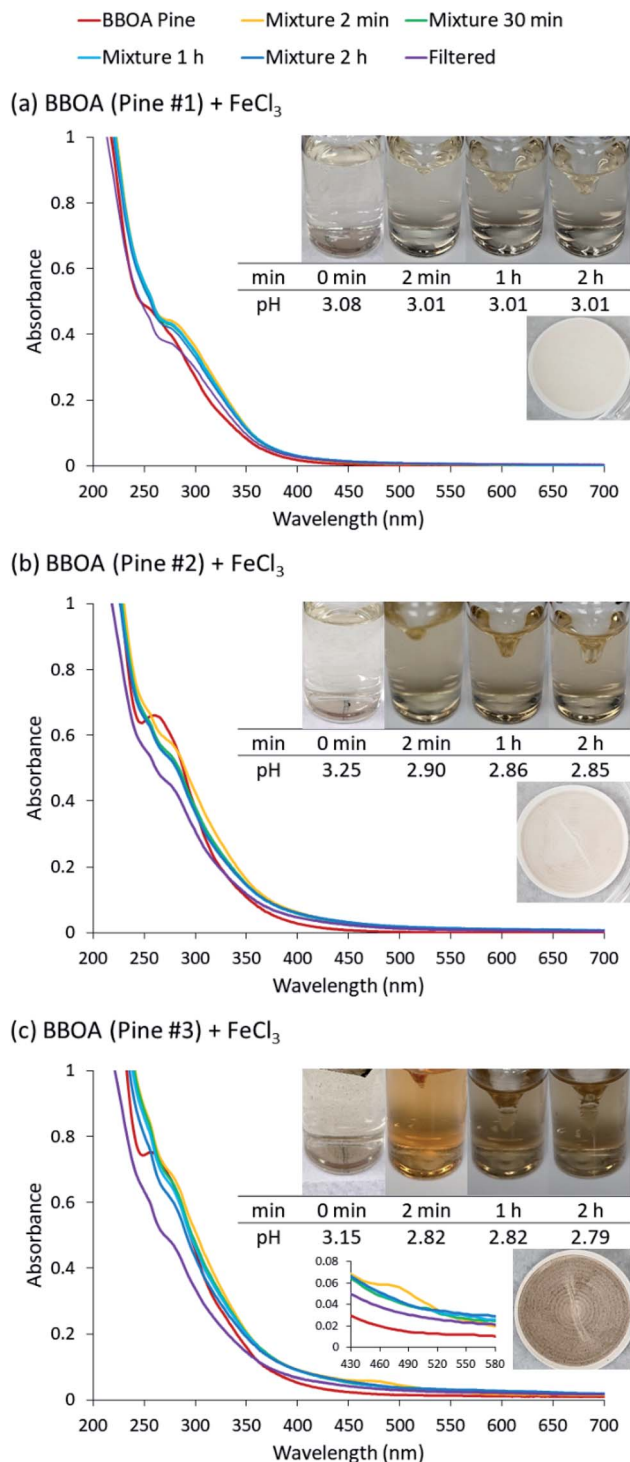
Fig. 20 UV-Vis absorption spectra of mixture of excess \text{Fe(III)} and BBOA extracts. Different colors of traces correspond to the spectra of BBOA before mixing (red), 2 min after mixing (orange), 30 min after mixing (green), 1 h after mixing (light blue), 2 h after mixing (dark blue), and filtered solution (purple). Reproduced from ref. 190 under Creative Commons License (CC BY-NC) from the Royal Society of Chemistry, © The Author(s), 2021.
