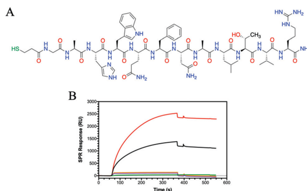
Fig. 3 (A) Chemical structure of thiolated Pep-1 for immobilization on SPR gold chip. (B) SPR sensorgrams for binding to Pep-1 using HA (5 kDa) (black) and the glycopolymers of P6 (red), P7 (green), P8 (purple) and P12 (orange) at 2000 nM.
