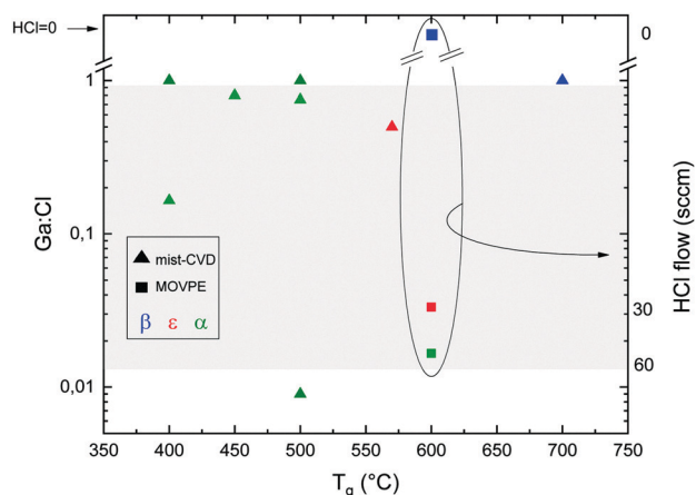
Fig. 1 Ga 2 O 3 phase on c -plane sapphire substrates as a function of the Ga:Cl ratio and temperature for the MOVPE (squares) and mist-CVD (triangles) techniques. Red symbols: \epsilon -Ga 2 O 3 . Blue symbols: \beta -Ga 2 O 3 . Green symbols: \alpha -Ga 2 O 3 . In the circle are summarized the data from ref. 42 using HCl along with O 2 and TEG; for these points the HCl flow is reported on the right y axis. The grey area represents reasonable Ga:Cl ranges for HVPE growth.
