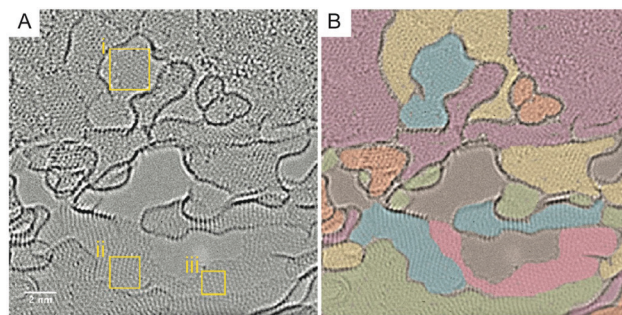
Fig. 11 (A) High-resolution image of mono- and few-layer graphene oxide at 700 °C imaged with an in situ TEM heating holder. (B) Overlaid color map represents layers of the material, showing turbostatic stacking and thicker and thinner regions. Reprinted with permission from (ACS Nano, 2016, 10, 7515–7522). Copyright (2016) American Chemical Society.
