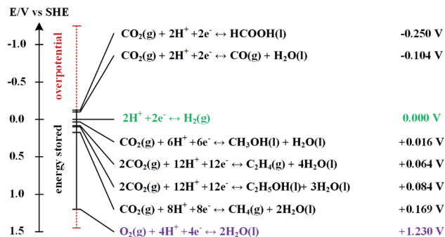
Fig. 2 Standard equilibrium potentials for hydrogen evolution half-cell reaction and several other half-cell reactions to reduce \text{CO}_2 into various products at 1 atm and 25 °C. Data presented was taken from Qiao et al. 27 (2014).
