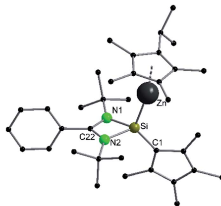
Fig. 3 Solid state structure of compound 3 . Hydrogen atoms are omitted for clarity. Selected bond lengths [Å] and angles [°]: Zn–Si 2.3056(9); Zn– \text{Cp}_{\text{centr}} 1.885(2); Si–N1 1.839(3); Si–N2 1.844(3); Si–C1 1.777(3); N1–C22 1.332(4); N2–C22 1.325(4); C1–C2 1.438(4); C1–C5 1.435(4); C2–C3 1.384(4); C3–C4 1.429(5); C4–C5 1.374(4); N1–C22–N2 106.3(3); N1–Si–Zn 109.99(8); N2–Si–Zn 106.14(9); C1–Si–Zn 122.55(10); N1–Si–C1 117.20(13); N2–Si–C1 118.84(13); Si–C1–C2 125.5(2); Si–C1–C5 128.0(2); C2–C1–C5 106.4(3).
