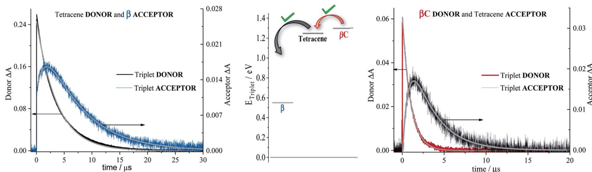
Fig. 5 Decay and rise dynamics of trimers (extreme left for \beta ; and extreme right for \beta C) in cyclohexane obtained by nanosecond TA for triplet sensitization measurements. Middle graph shows the triplet energy for samples and sensitizers.
