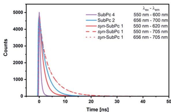
Fig. 8 Fits of fluorescence decays obtained by the time correlated single photon counting method of monomer-SubPc 4 ( 1.5 \times 10^{-6} \text{ M} ), dimer-SubPc 2 ( 1.5 \times 10^{-6} \text{ M} ), and syn -SubPc 1 ( 1.5 \times 10^{-6} \text{ M} ) in argon purged toluene. The excitation and emission wavelengths were as given in the legend.
