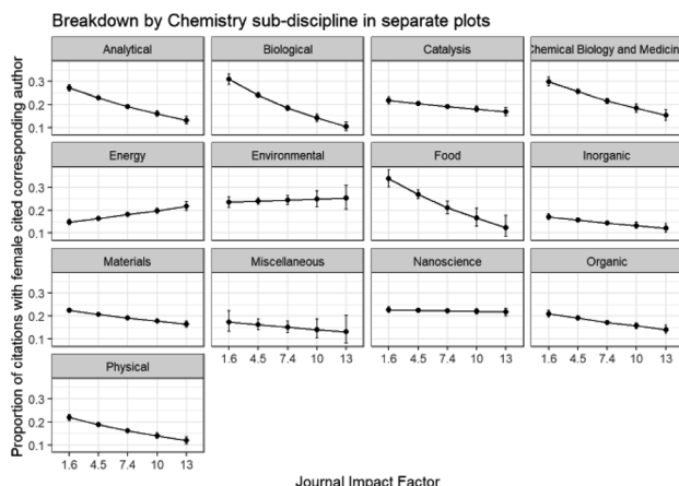
Fig. 30 Binomial GLM model of corresponding author gender of citations, chemistry sub-discipline and journal impact factor (Model: CitedCorrAuthorGender ~ Category * ImpactFactor). ANOVA \text{Pr}( > \text{Chi} ) : category is highly significant ( 3.26 \times 10^{-66} ); ImpactFactor is highly significant ( 1.96 \times 10^{-17} ); category: ImpactFactor interactions are highly significant ( 2.49 \times 10^{-14} ).
