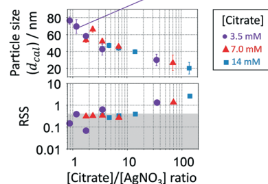
Fig. 10 Effect of the [citrate]/[ AgNO_3 ] ratio of the sequential additions in the growth-stage. A. UV-vis spectra, peak location and optical density of particles in R5. B. Calculated average particle size and spherical degree (RSS) using the Mie theory-based algorithm. For smaller particle sizes, the number of growth reactors should be reduced. Conditions: nucleation reactor → refer to Fig. 5 growth reactors → same as Fig. 6 and 7 except for changes in the citrate/ AgNO_3 ratio.
