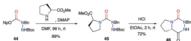
Scheme 16 Aza-DKP synthesis from an activated carbamate.
