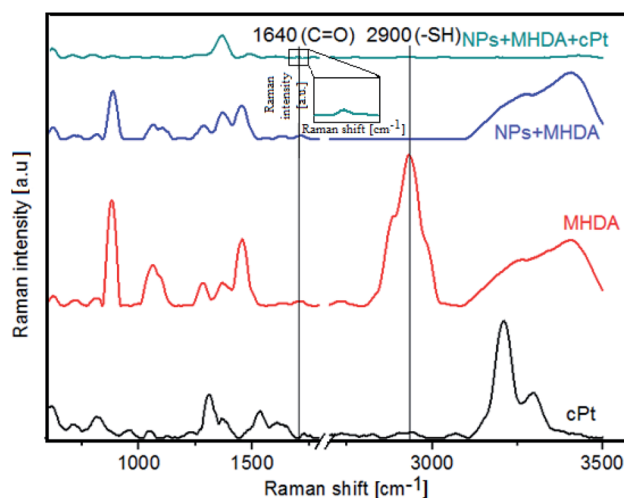
Fig. 9 Raman spectra of: cPt (black spectrum), the pure MHDA (red spectrum), the \text{Fe}_3\text{O}_4@SiO_2@Au + MHDA (blue spectrum), \text{Fe}_3\text{O}_4@SiO_2@Au + MHDA + cPt (green spectrum).
