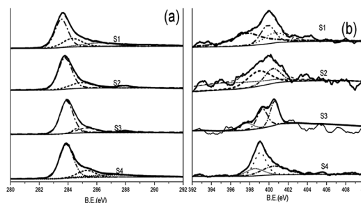
Fig. 3 XPS spectrum of (a) C 1s spectrum and (b) N 1s spectrum of NHCSSs.
