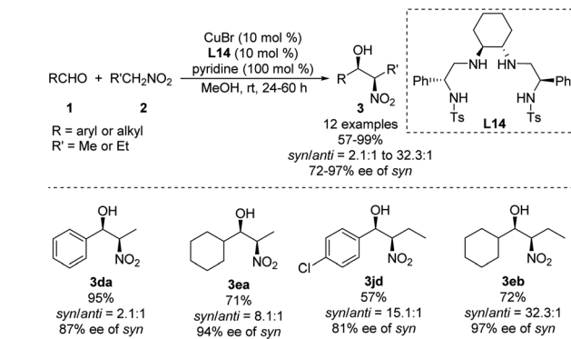
Scheme 24 Syn -selective asymmetric Henry reaction catalyzed by \text{Cu-L14} .
