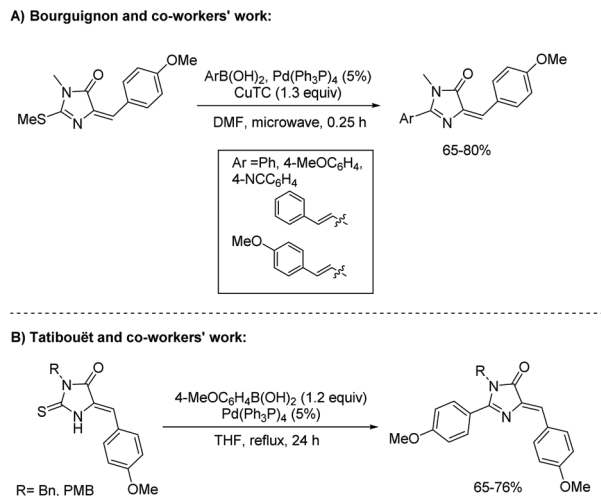
Scheme 20 Conversion of thiohydantoin to 2-aryl-imidazol-4-one.
