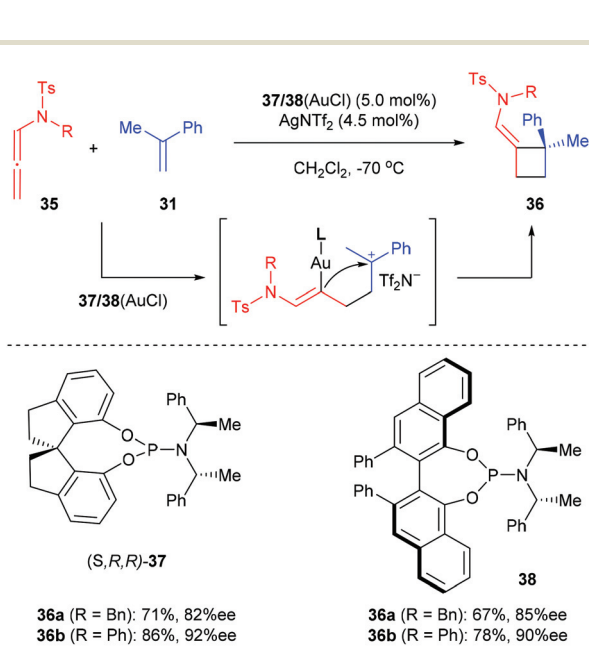
Scheme 10 Au(I)-Catalyzed intermolecular [2 + 2] cycloaddition.
