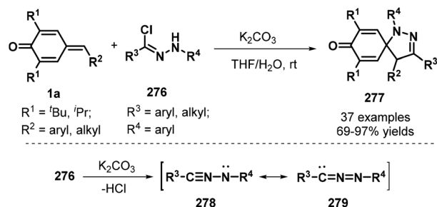
Scheme 61 [3 + 2] annulation of p -QMs with hydrazonyl chlorides.
