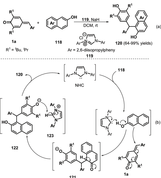
Scheme 24 NHC-Catalyzed 1,6-addition of 2-naphthols to p -QMs.
