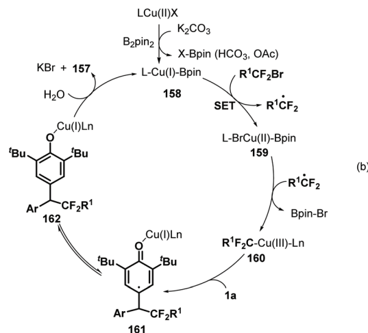
Scheme 32 1,6-Hydrodifluoroacetylation of p -QMs.
