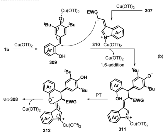
Scheme 67 [4 + 2] annulation toward chromans.
