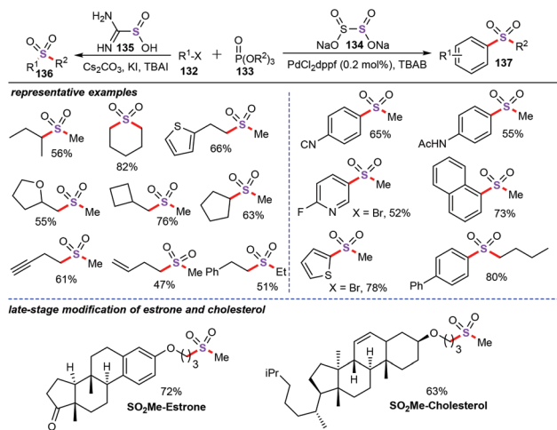
Scheme 50 General sulfone construction via SO 2 surrogate control.
