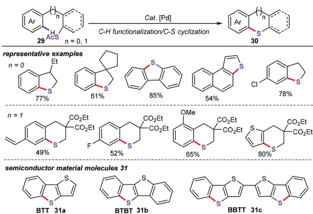
Scheme 11 Palladium-catalyzed C–S cyclization reaction.
